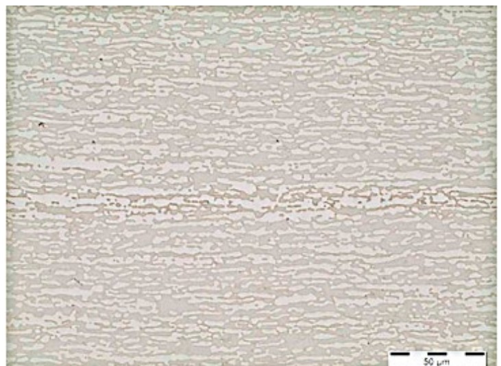
Example of DX2507 microstructure (ferrite in grey, austenite in white) - no intermetallic phases detected.
