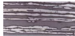
Microstructure of DX1803/DX2205 (dark areas represent the ferritic phase)
