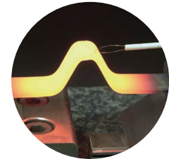
Thermal fatigue bench
